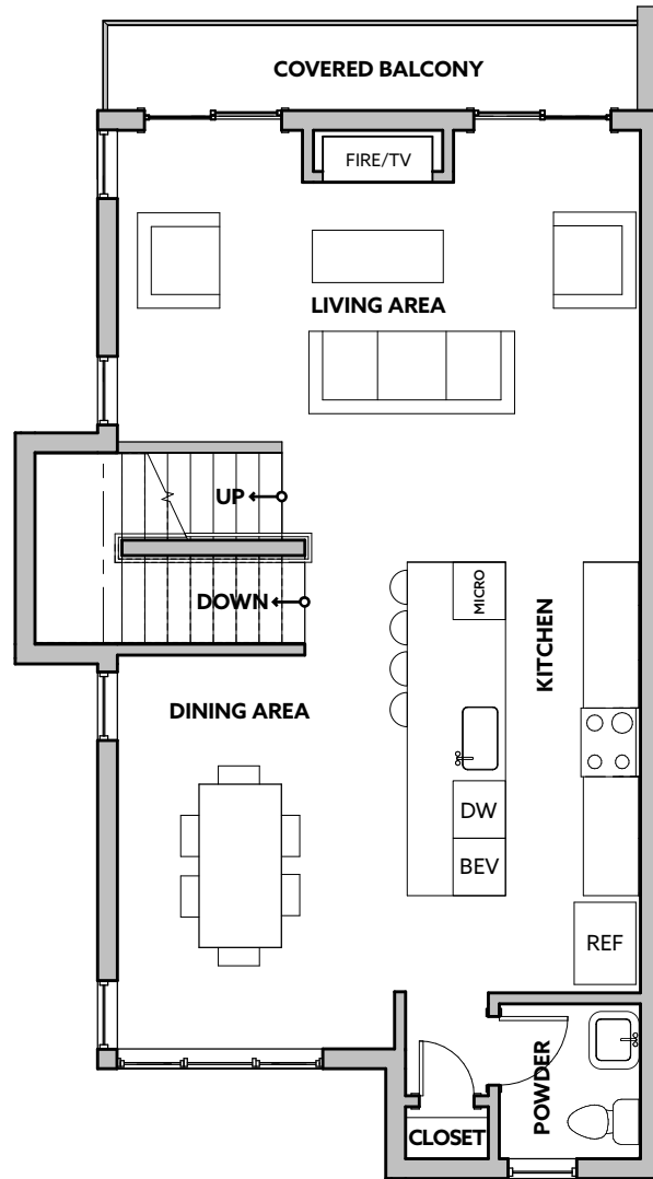
2ND FLOOR 9' CEILING
